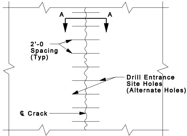
Longitudinal or Transverse Crack
